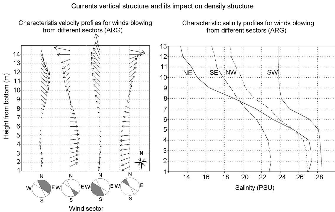
Figura 10: Left: Characteristic current profiles for winds blowing from different sectors as derived from ADCP data collected at ARG (see location in Figure 1). Right: Composites of salinity profiles in the vicinity of ARG for winds blowing from the NE, SE, SW and NW directions. For winds with a dominant component perpendicular to the estuary axis, the response is in the form of vertically decaying currents, whereas for winds with a dominant component along the estuary axis, a marked inversion in current direction between upper and lower levels occurs. The vertical density structure responds to currents: for north-easterly/south-westerly winds an extension towards the southern/northern coast of the surface front and an enhancement of the stratification along that coast occur; only for south-easterly wind stratification can be broken. Adapted from Simionato et al. (2007), reprinted with permission from Elsevier.
