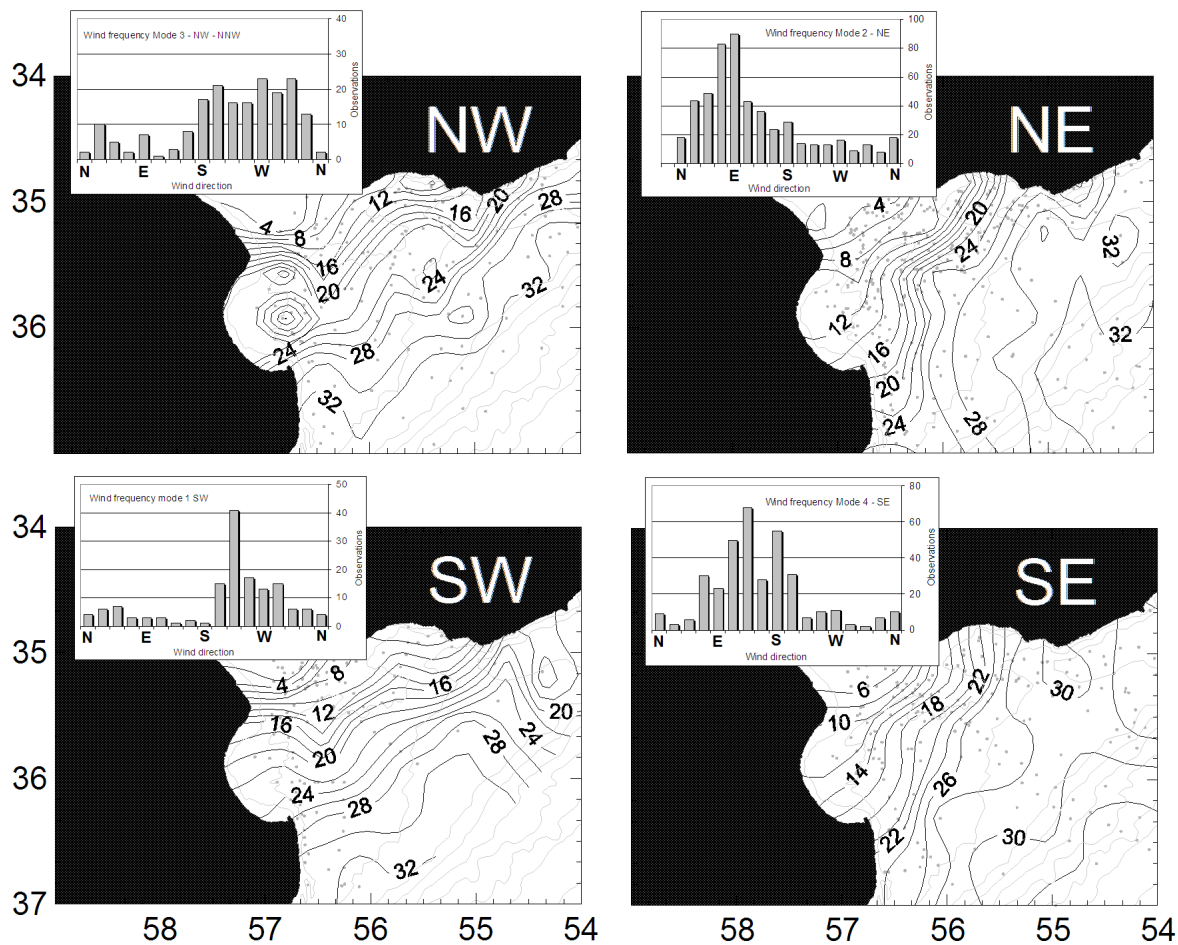
Figura 11: Composites of observed surface salinity fields (PSU) for winds blowing from different sectors. CTD data from oceanographic cruises and winds at Pontón Recalada station (close to PON, figure 1) were used. The insets show the wind histograms corresponding to the data composed. The response to winds can be observed in composites collected over different times of the year, indicating that it is very fast and that variability dominates in this estuary. From Meccia et al. (2013), reproduced with permission from the Coastal Education and Research Foundation, Inc.
