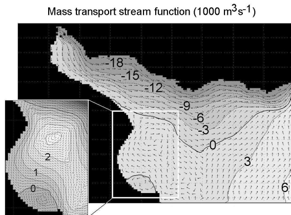
Barotropic (vertically averaged) circulation of the Río de la Plata
