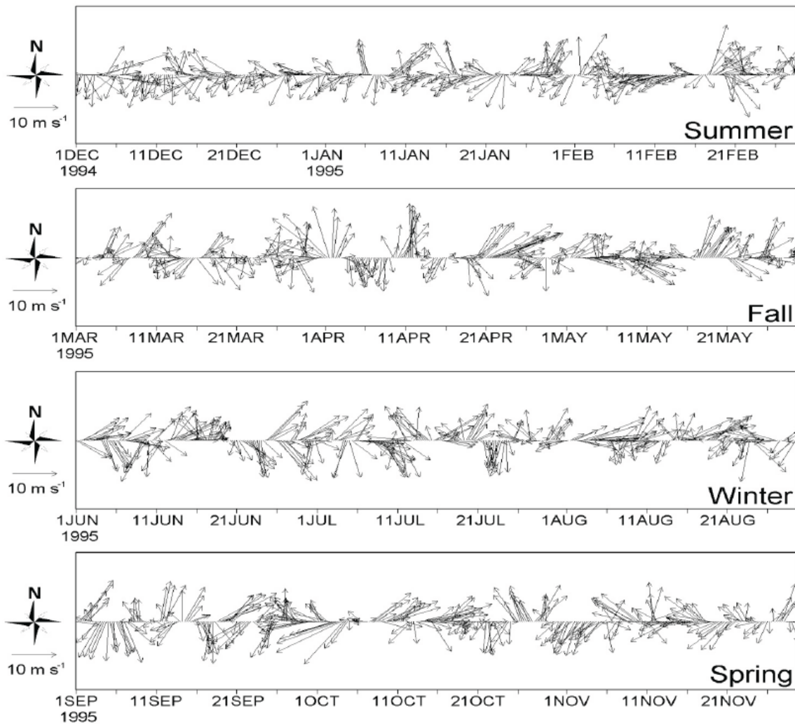
Figura 5: Four-daily wind vectors stick diagrams for the four seasons of an arbitrary year (in this case, 1995) from the NCEP/NCAR reanalysis at 35.2°S 54.37°W. The main feature of wind variability in the region is their alternancy from northeast to southwest; north-easterlies are more frequent in summer and south-westerlies, in winter. Reprinted from Simionato et al. (2008) with permission from Elsevier.
