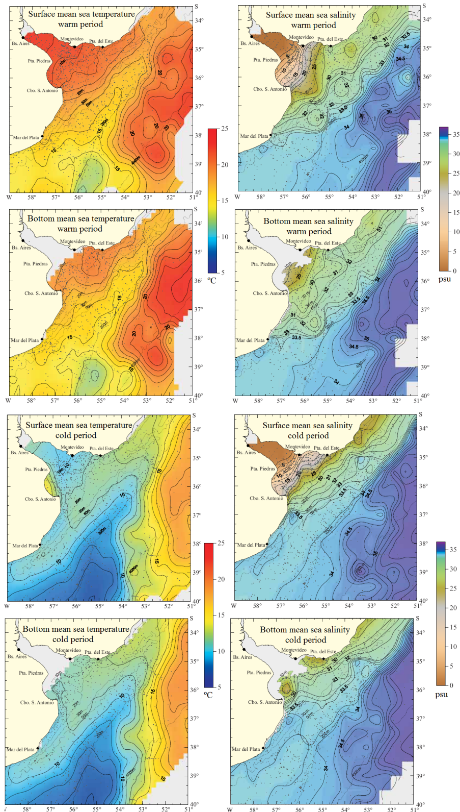
Figura 6: Mean sea temperature (left panels) and salinity (right panels) for the warm and cold seasons for the surface (upper panel) and bottom (lower panel) layers. All the figures correspond to a normal (around the mean) continental discharge condition. The figure shows the most characteristic seasonal pattern of the salinity field in the RdP, with the freshwater mass extending offshore along the northern coast of the estuary in winter and retracting south-westward in summer. From Guerrero et al. (2010).
