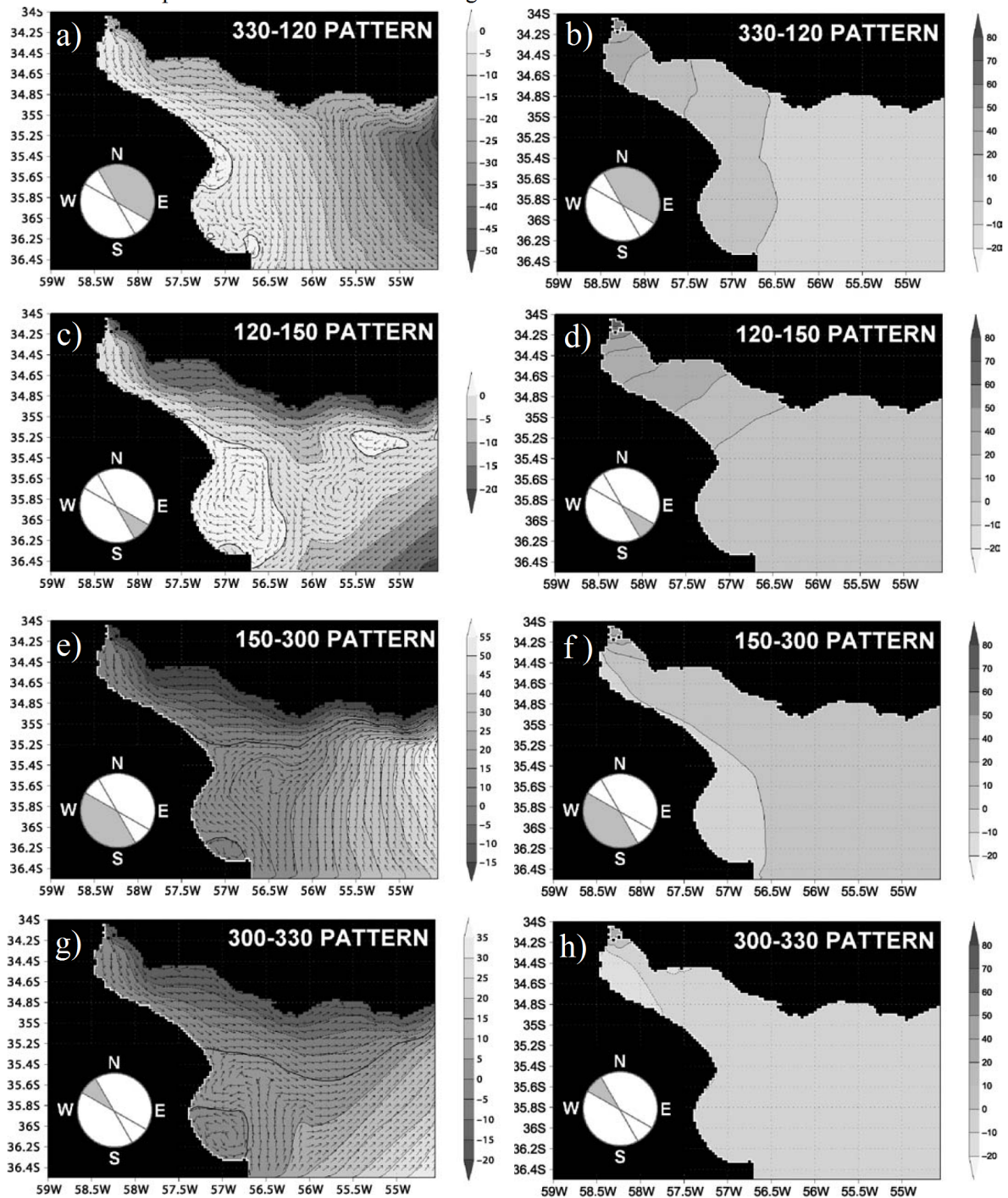
Figura 9: Main residual transport stream function (in thousands of \text{m}^3\text{s}^{-1} ) patterns (left panel) and mean sea surface elevation (cm) patterns (right panel) at the RdP estuary related to winds blowing from different sectors. The magnitude of the transport between two isolines equals the difference between their associated values. The RdP is very sensitive to the winds and behaves as a semi-enclosed basin. For winds from the southeast/northwest the circulation induces an increment/reduction of the level at the upper estuary. For winds with a component perpendicular to the estuary axis the circulation is characterized by changes over the northern and southern coast of the estuary. Adapted from Simionato et al. (2004b), reprinted with permission from Elsevier.
