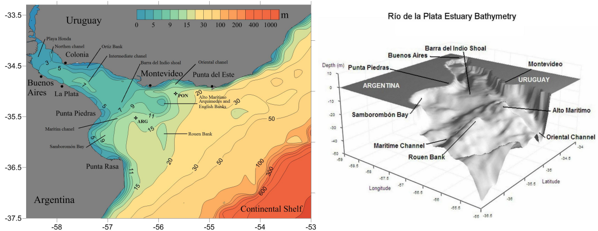
Figura 1: Bathymetry of the Río de la Plata Estuary (in m) and main geographical and topographical features in a 3-dimensional view (right) and a plant view with isobaths (left). Note that in the 3-d view, vertical and horizontal scales are different. The points denoted as ARG and PON show the sites where ADCP data were gathered during the FREPATA Project. Adapted from Moreira (2016) and Simionato et al. (2008) reprinted with permission from Elsevier.
