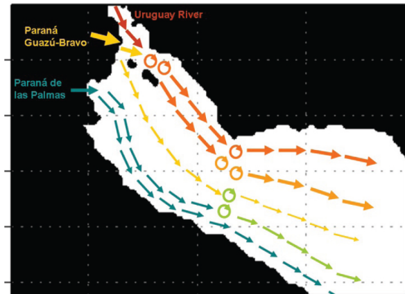
Figura 13: Schematic representation of the path of the water masses of the RdP Estuary main tributaries. The Uruguay, Paraná Guazú-Bravo and Paraná de las Palmas waters tend to flow along the northern, central and southern portions of the estuary, respectively, even though lateral mixing occurs, particularly to the northeast of the Martín García and Oyarvide islands and downstream Colonia del Sacramento, where the orientation of the coast changes. Reprinted from Simionato et al. (2009).
