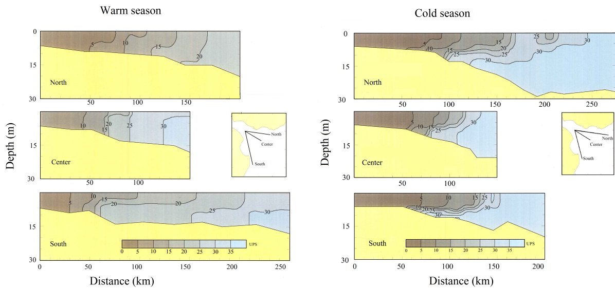
Figura 7: Vertical salinity profiles (in PSU) in the RdP along three different sections (a) north, (b) central and (c) south, for the warm (left) and the cold (right) seasons. The extension and changes in the stratification during the year can be appreciated, in particular along the northern section. From Guerrero et al. (1997b).
