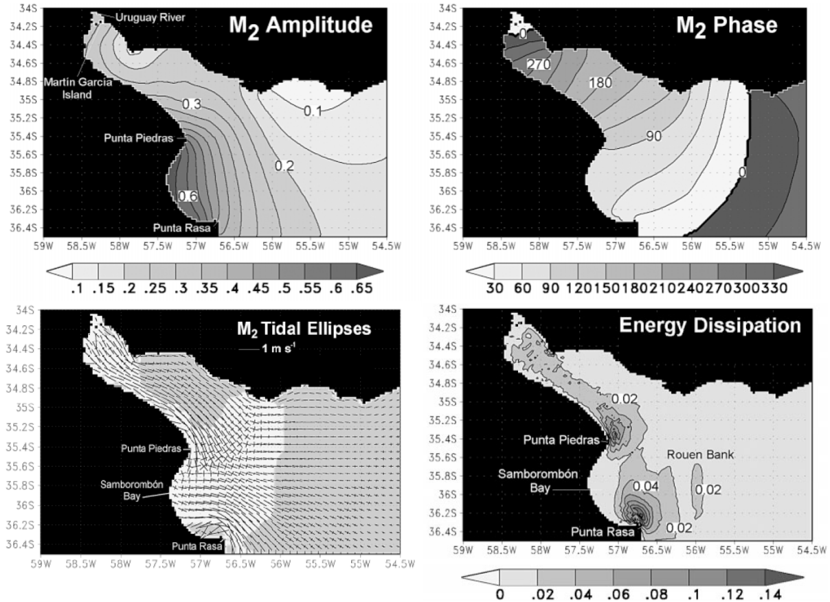
Figura 4: Tidal amplitude (m) and phase ( ^{\circ} ) for the M_2 tidal constituent (upper left and right panels), current ellipses ( \text{ms}^{-1} , gray colour indicates clockwise rotation and white colour indicates anti-clockwise rotation, lower left panel) and energy dissipation by bottom friction (in \text{wm}^{-2} , lower right panel). The figure shows how the wave propagates upstream as a Kelvin wave and that it loses its energy by bottom friction, particularly at the tips of Samborombón Bay and along the southern coast of the estuary. Adapted from Simionato et al. (2004a), reproduced with permission from the Coastal Education and Research Foundation, Inc.
