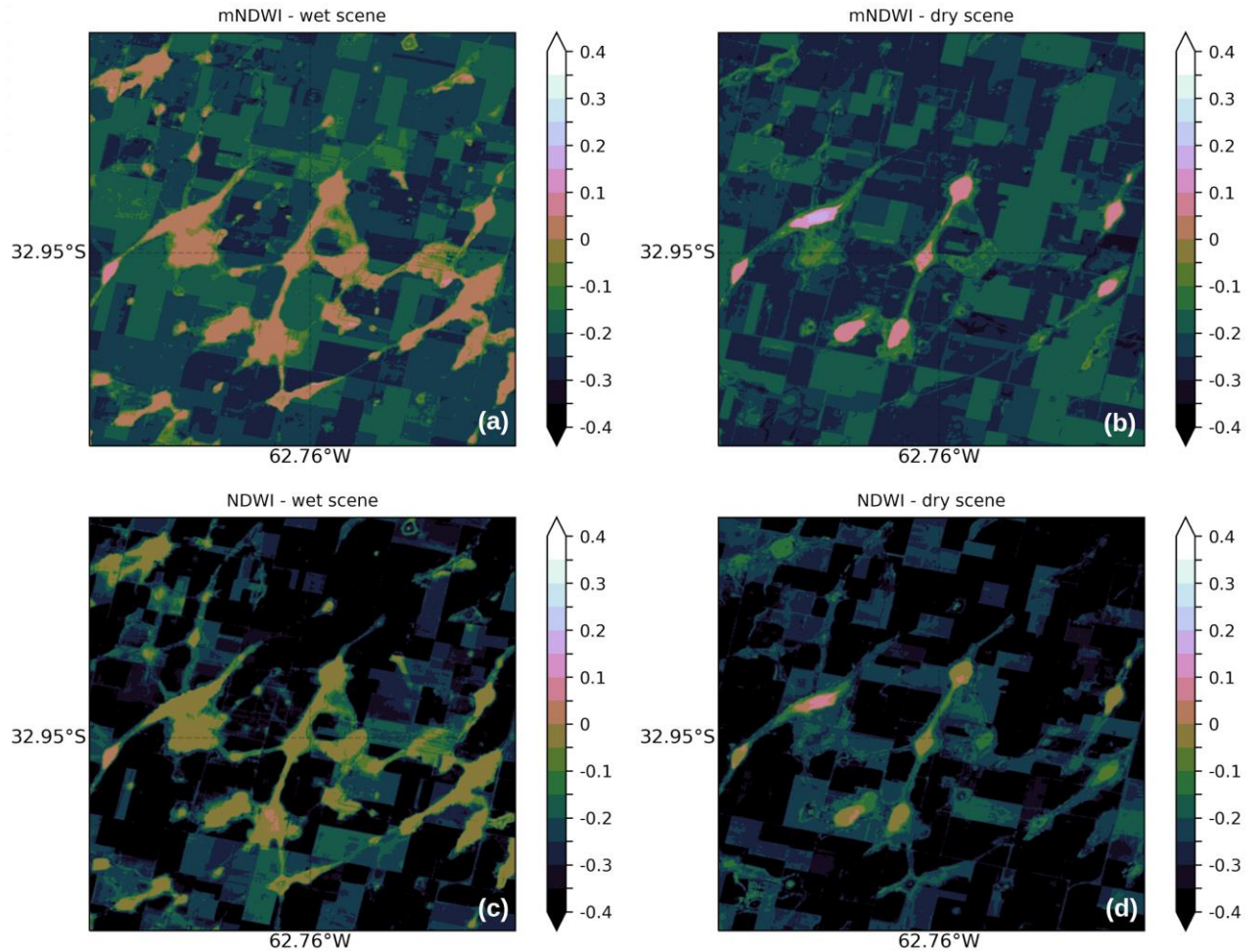
Figure 2: Mapping of the mNDWI and NDWI indices over the study site, based on Landsat 8 scenes from 7 January 2020 (wet scene) and 9 January 2021 (dry scene). (a): mNDWI, wet scene. (b): mNDWI, dry scene. (c): NDWI, wet scene. (d): NDWI, dry scene.
